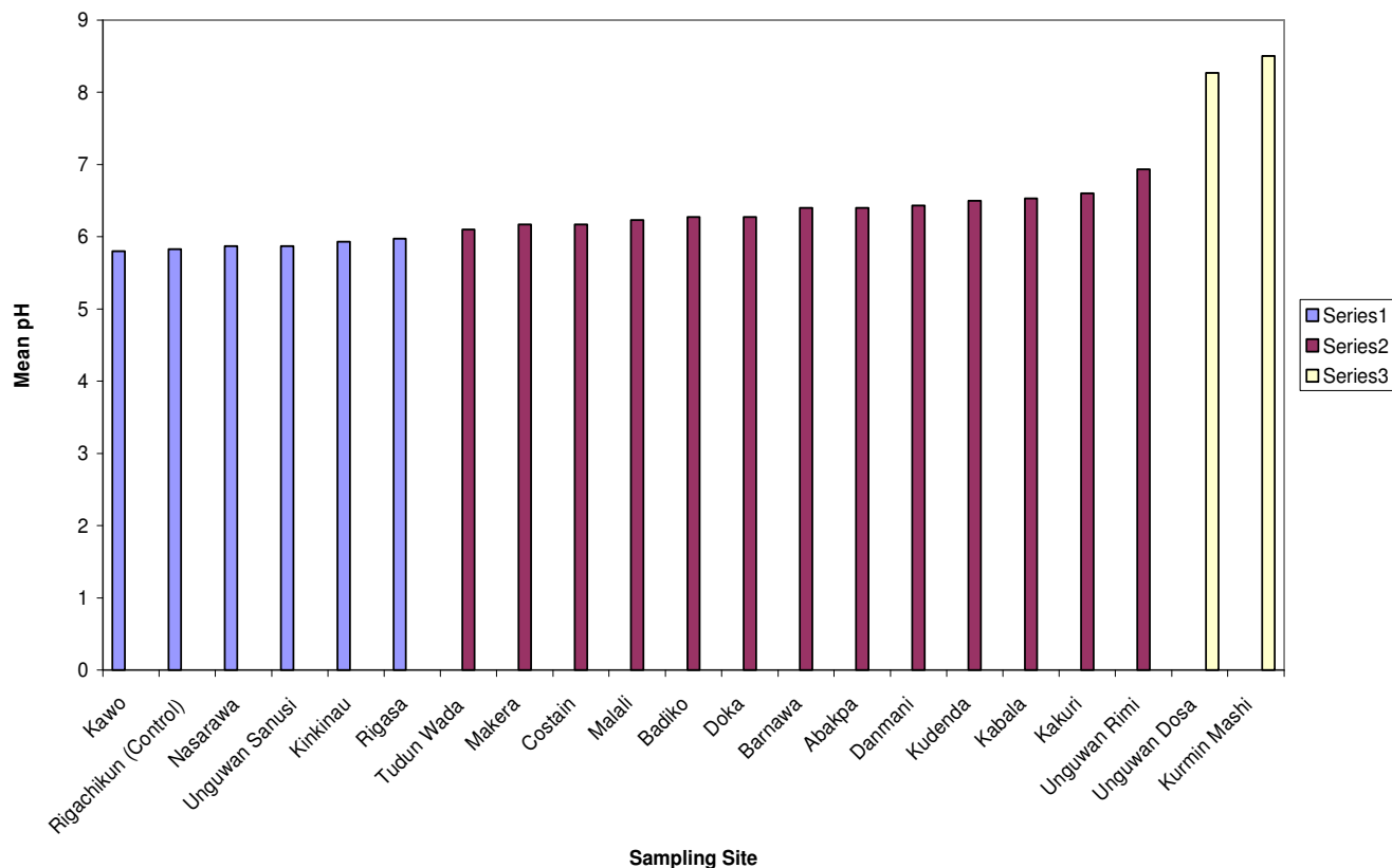
Figure-2 A mean plot for Soil pH
